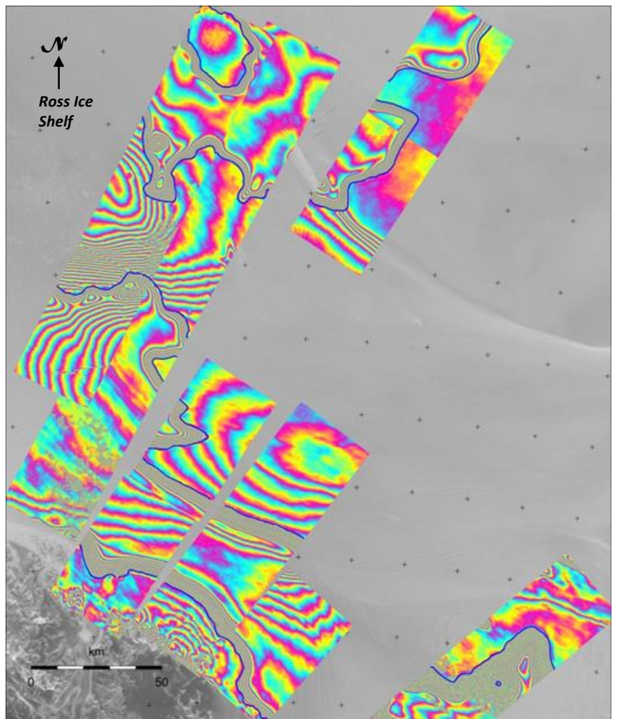
ABOVE: Grounding Line Location (blue line) at the Ross Ice Shelf derived from repeat pass TerraSAR-X data acquired in 2012 (processing by DLR). Ice deformation at the grounding zone is apparent as a dense fringe belt separating the floating and grounded ice. The grounding line product will consist of a polygon representing the inland limit of tidal flexure.
