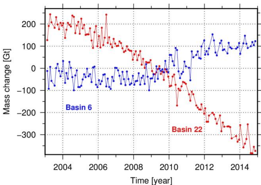
ABOVE: Illustration of the Gravimetry Mass Balance data products (processing by TUDr / TUM).
