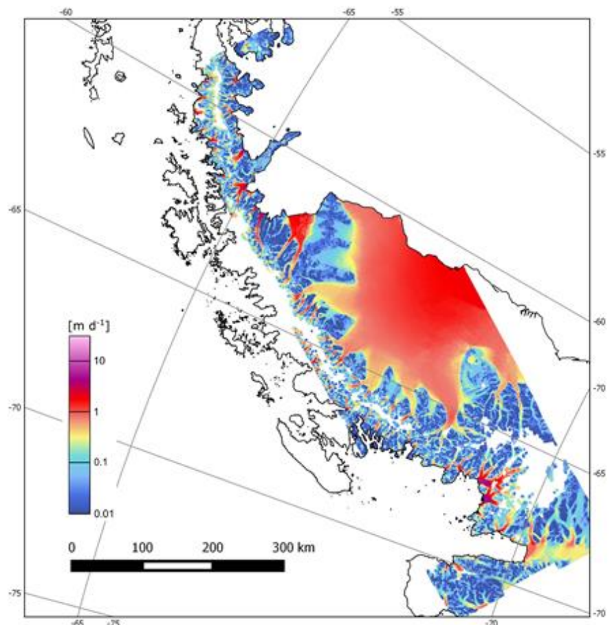
ABOVE: Ice velocity map for Antarctic Peninsula from Sentinel-1 data acquired in June 2015 (processing by ENVEO).
